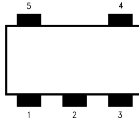
DBV Package 5 Pin SOT-23 Top View
