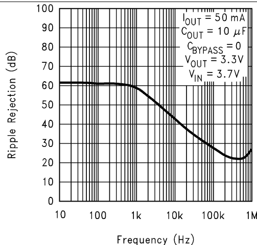
Figure 8. Ripple Rejection
