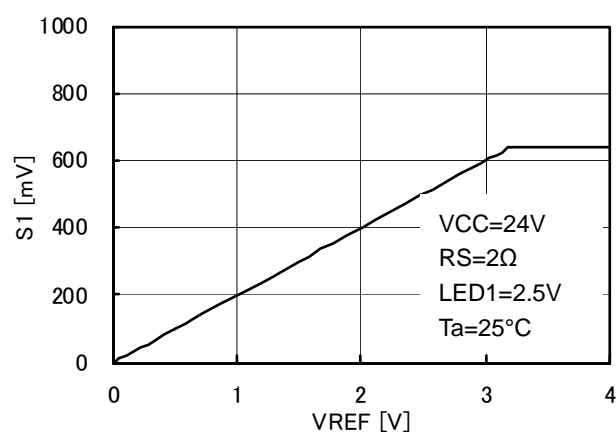
Figure 9. V_{REF} v.s. S_x
