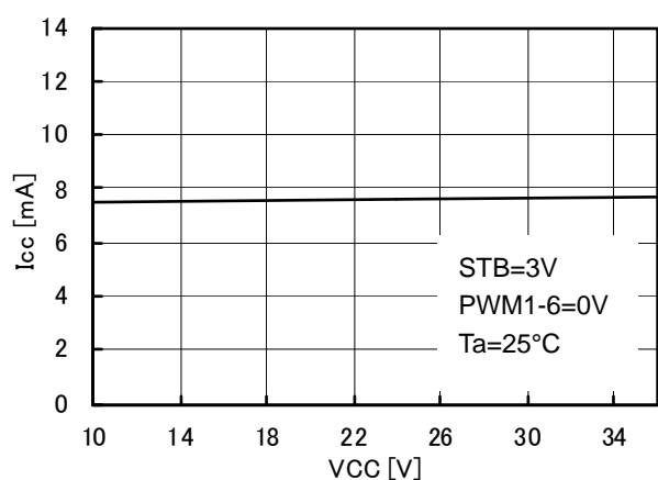
Figure 6. Circuit current
