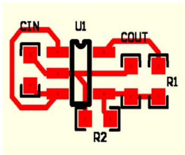
Figure 6. Adjustable Mode
