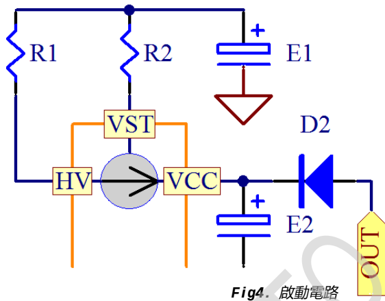
Fig4. 啟動電路
